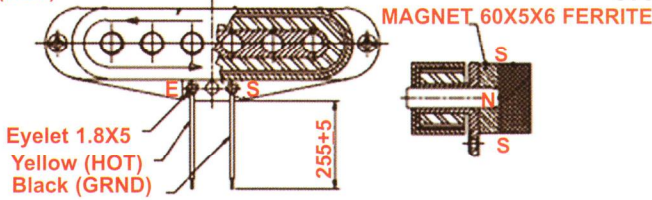
MMPSS-M/BK Single Coil Pickup (Middle) Great Tone / Available In Black or White
