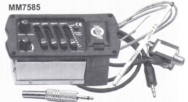
Mighty Mite® 3 Band Active EQ, Plus Volume Control, w/ Slim Jim® Bridge Mount Pickup.
