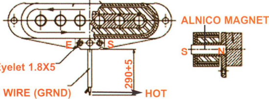
MMVPSS-M/BK ALNICO Single Coil Pickup (Middle) Vintage Tone / Available In Black or White
