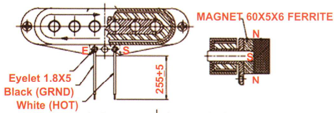
MMPSS-F/BK Single Coil Pickup (Front) Great Tone / Available In Black or White
