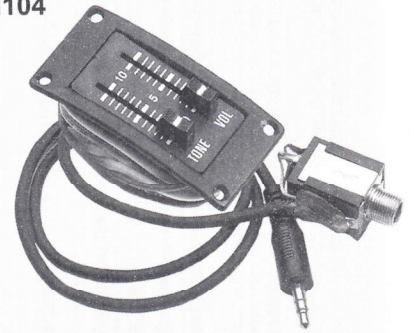
Mighty Mite® Transducer Pickup, w/ Tone Controls.
