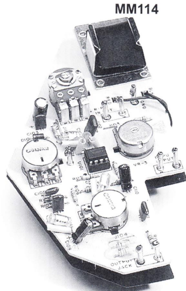
Mighty Mite® Active Bass Control Pre-Amp, w/ Master Volume, Fade, Treble & Bass.
