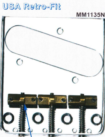
New USA Retro-Fit Tele Bridges with Brass Saddles
