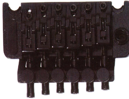
MMBL002B Floyd Rose® Style Bridge
