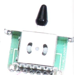
MM503 Mighty Mite® Strat® Replacement 5 Way Switch With Black Knob (Double Pole)
